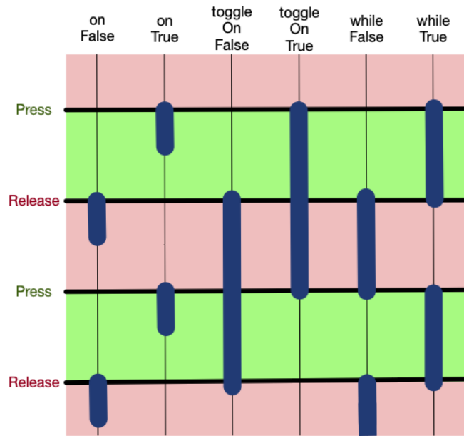
onTrue starts when a button is pressed and usually ends on its own. whileTrue starts when the button is pressed and runs until it is released. toggleOnTrue turns on or off in alternation every time the button is pressed. onFalse , whileFalse , and toggleOnFalse do the same, but when the button is released.
